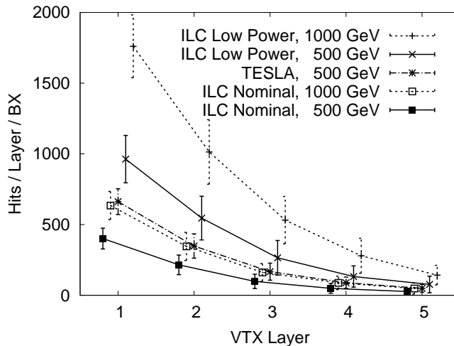
Figure 3: Number of hits on the vertex detector for various beam parameter sets
