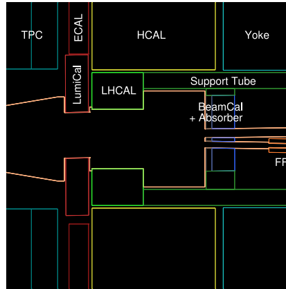
Figure 2: Design of the forward region (compressed view 1:2)
