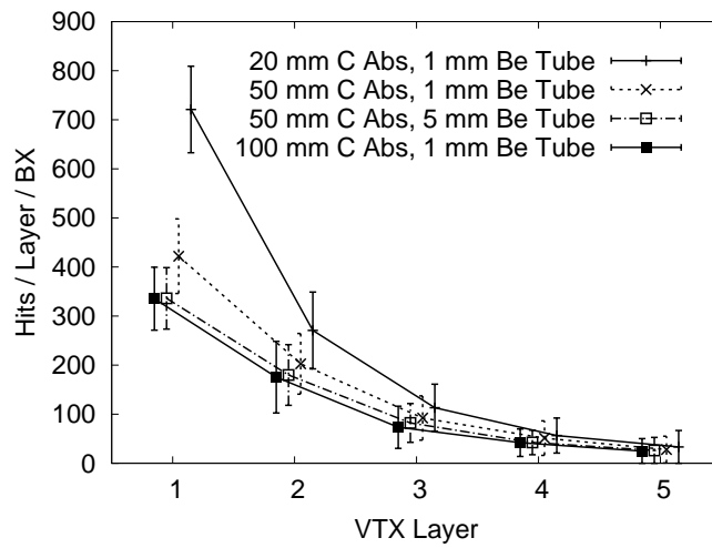
Figure 4: Number of hits on the vertex detector in relation to the thickness of the low-Z absorber
