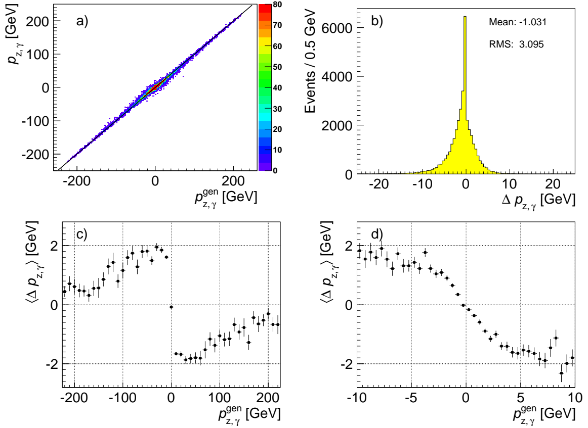
Figure 4: Fitted photon momentum p_{z,\gamma} plotted against the true momentum p_{z,\gamma}^{\text{gen}} of the most energetic ISR+beamstrahlung photon combination in the event (a), distribution of the difference \Delta p_{z,\gamma} = \text{sign}(p_{z,\gamma}^{\text{gen}}) \cdot (p_{z,\gamma} - p_{z,\gamma}^{\text{gen}}) (b), and mean difference \langle \Delta p_{z,\gamma} \rangle versus the true momentum for the full range of p_{z,\gamma}^{\text{gen}} (c) and small values |p_{z,\gamma}^{\text{gen}}| \leq 10 GeV (d).
