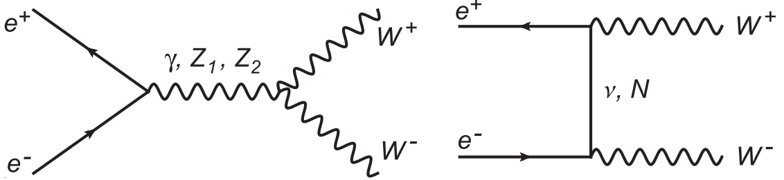
FIG. 1: Feynman diagrams.
